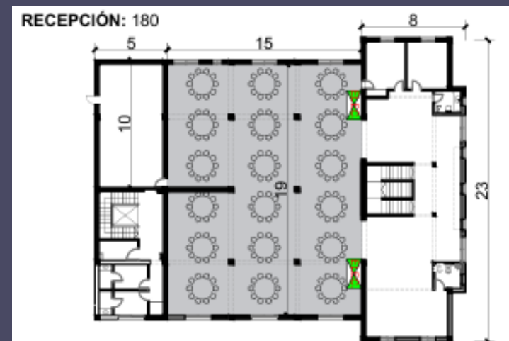
PLANO RECEPCIÓN
